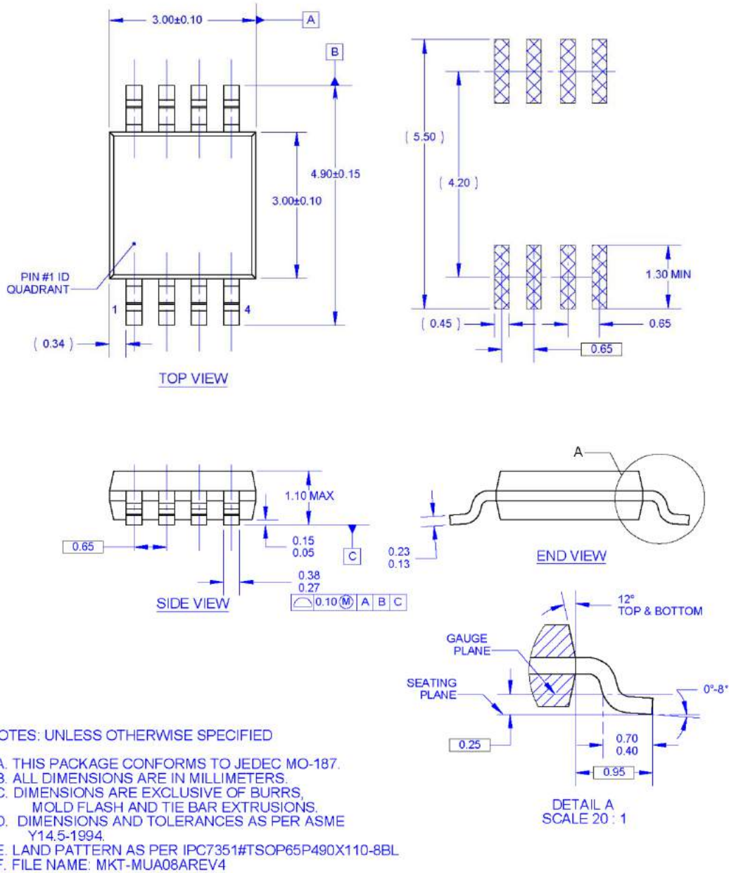
Figure 34. 8-Lead, Molded Small-Outline Package (MSOP)
