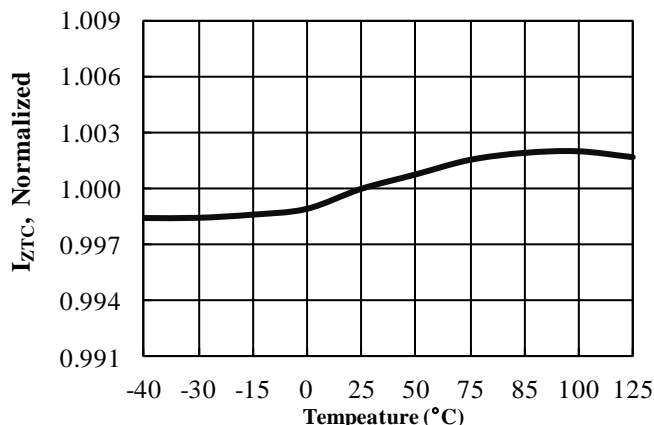
Figure 16. Dynamic trigger current threshold (I ZTC ) vs. Temperature
