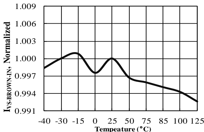
Figure 18. Brown In Threshold Current (I VS-BROWN-IN ) vs. Temperature
