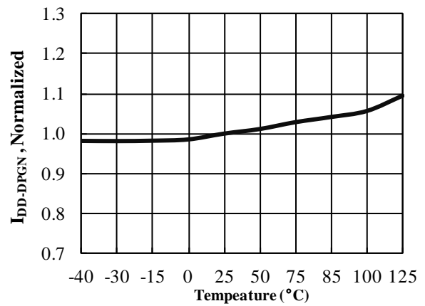
Figure 6. Deep Green Mode Operation Current (I DD-DPGN ) vs. Temperature
