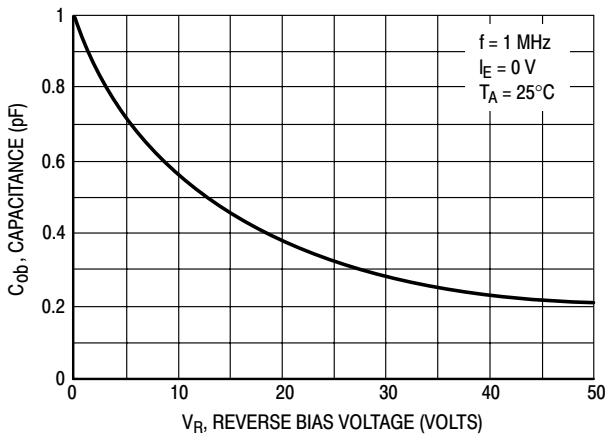
Figure 14. Output Capacitance
