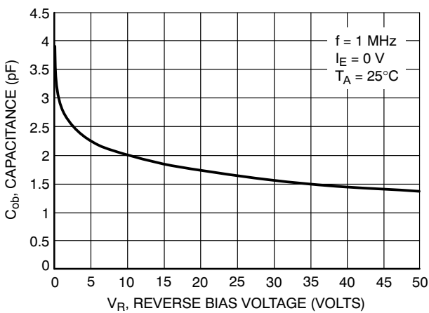
Figure 29. Output Capacitance
