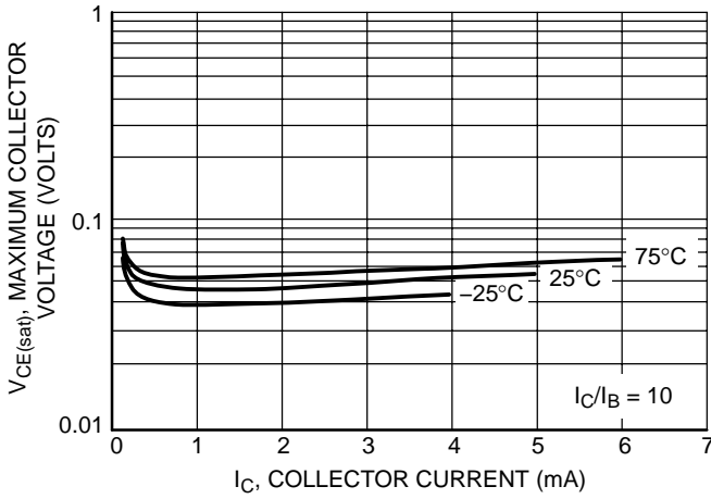
Figure 23. Maximum Collector Voltage vs. Collector Current
