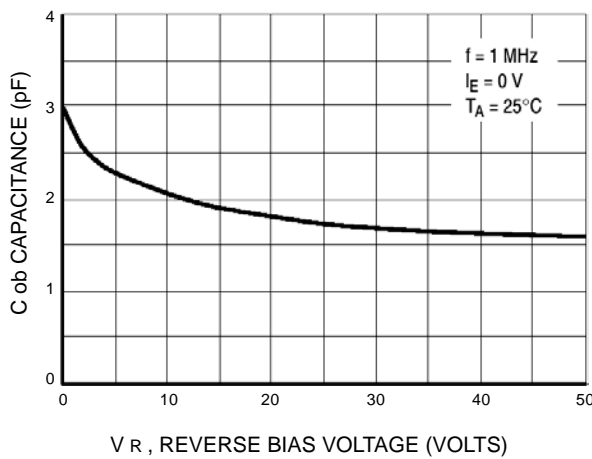
Figure 4. Output Capacitance
