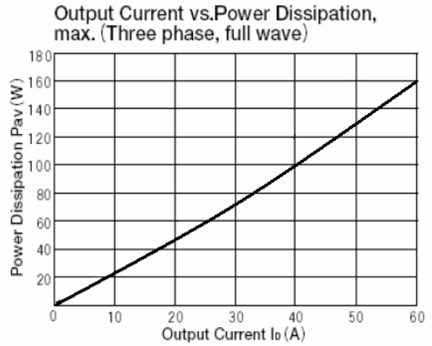
Fig.2. Output Current vs. Power Dissipation
