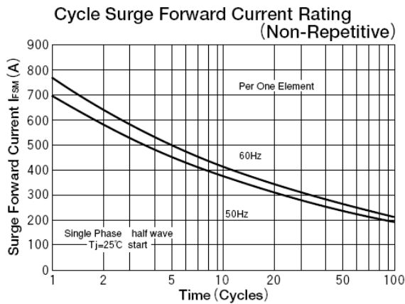
Fig.3. Surge overload characteristics vs. time
