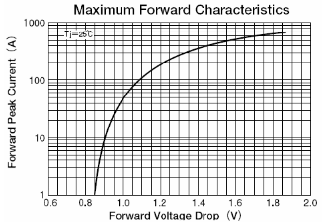
Fig.4. Forward characteristics of a diode arm
