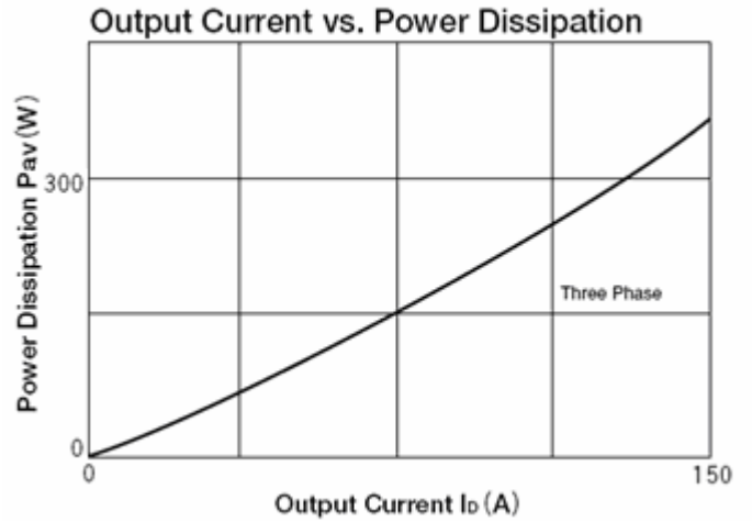
Fig.2 Power dissipation vs. Power Dissipation
