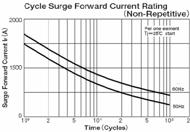
Fig.3. Surge overload characteristics vs. time
