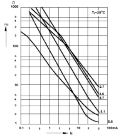
Dynamic resistance versus Zener current
