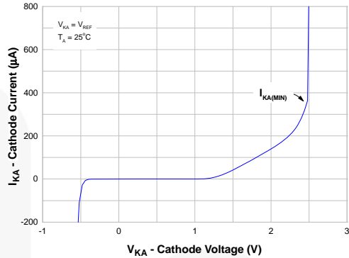
Figure 11. Cathode Current vs. Cathode Voltage
