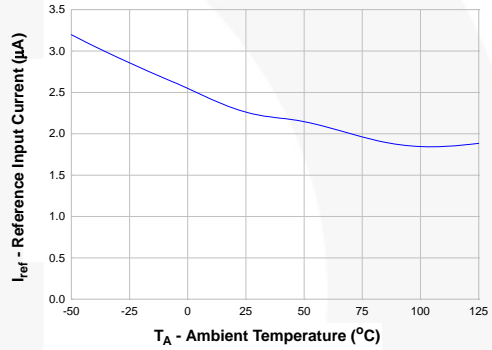
Figure 13. Reference Input Current vs. Ambient Temperature
