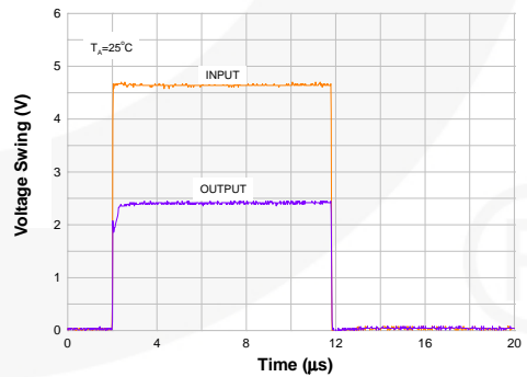
Figure 15. Pulse Response
