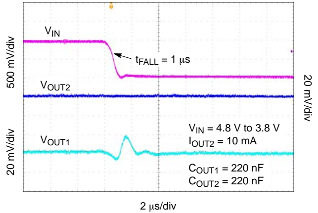
Figure 32. Line Transient Response – Falling Edge, V EN1 = V IN , V EN1 = 0 V, V OUT1 = 3.3 V, I OUT1 = 10 mA
