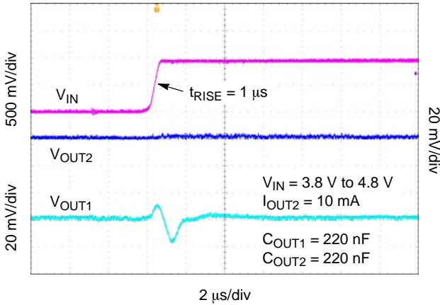
Figure 31. Line Transient Response – Rising Edge, V EN1 = V IN , V EN1 = 0 V, V OUT1 = 3.3 V, I OUT1 = 10 mA
