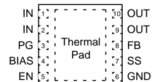
DFN10-3x3-0.5P
