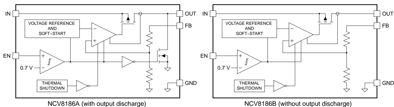
Figure 2. Internal Block Diagram
