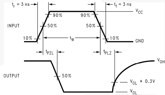
Figure 5. AC Waveforms
