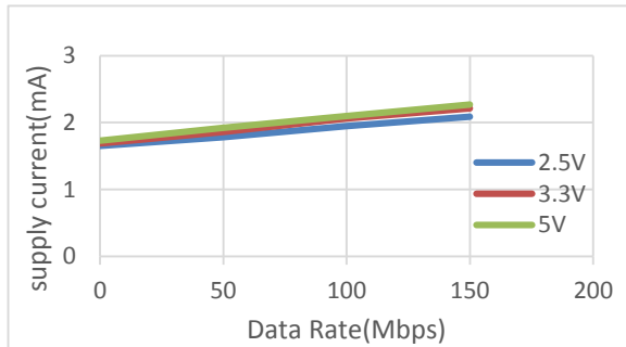
Figure 2.1 NSi8120 VDD1 Supply Current vs Data Rate
