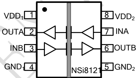
Figure 6.2 NSi8121N Package
